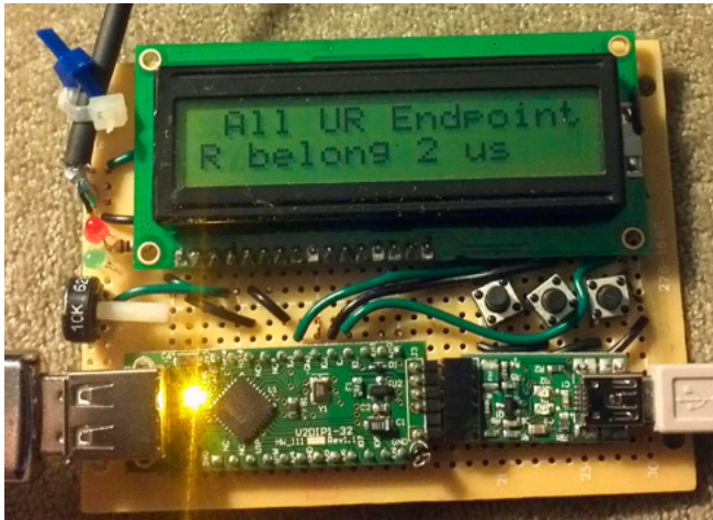
Figure 1. USB Impersonator
